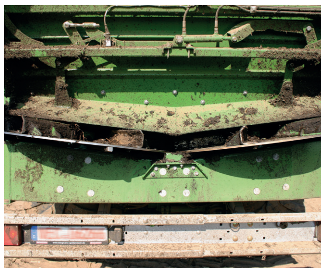
Fig. 6: The V-Spread discs in chevron-style arrangement
