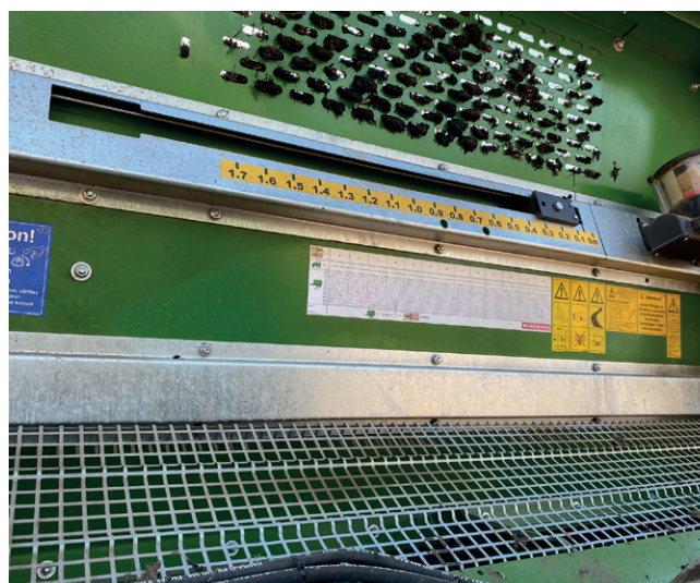
Fig. 5: This scale on the headboard indicates the current aperture of the slurry gate upstream of the beaters
