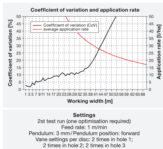
Fig. 10: Coefficient of variation relative to the work width in muck spread at a rate of 30 t/ha
