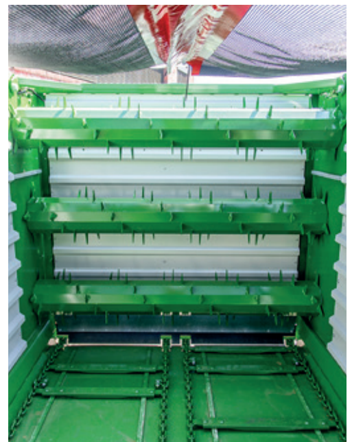
The S-model dosing unit with three standard dosing rollers ( CAREX 370 S / CAREX 410 S ).
